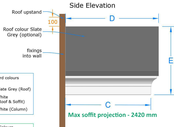
White Portico & Slate Grey Roof (incl standard sized fluted columns)
