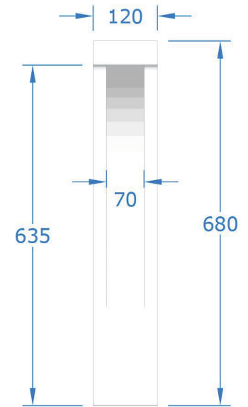
Front Elevation
