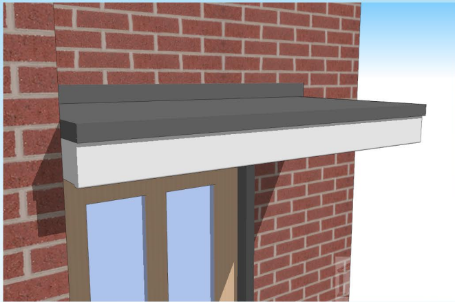
Left-hand Corner-fit with Standard Abutment detail (also available as Right-hand)
