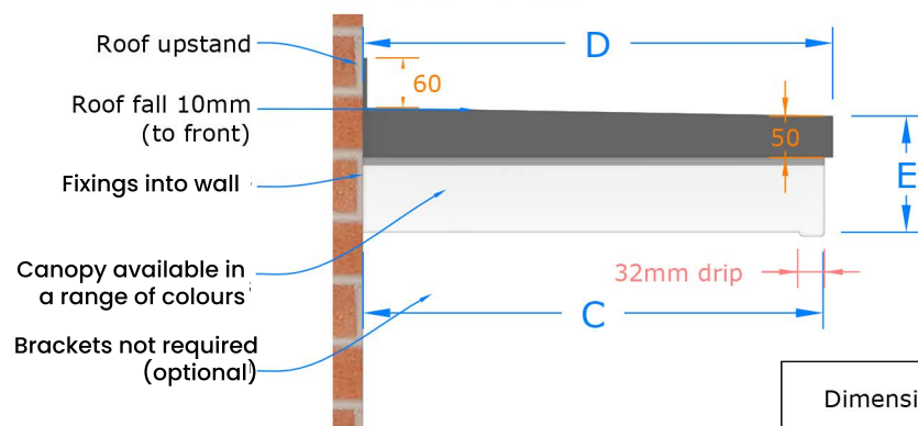
Side Elevation
